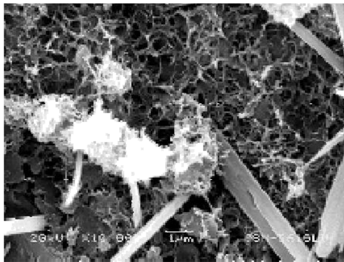
C-S-H 凝胶
