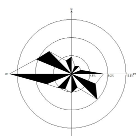
七月静风 2.82%
