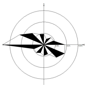
春季静风 0.82%
