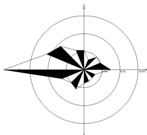
十月静风 2.82%
